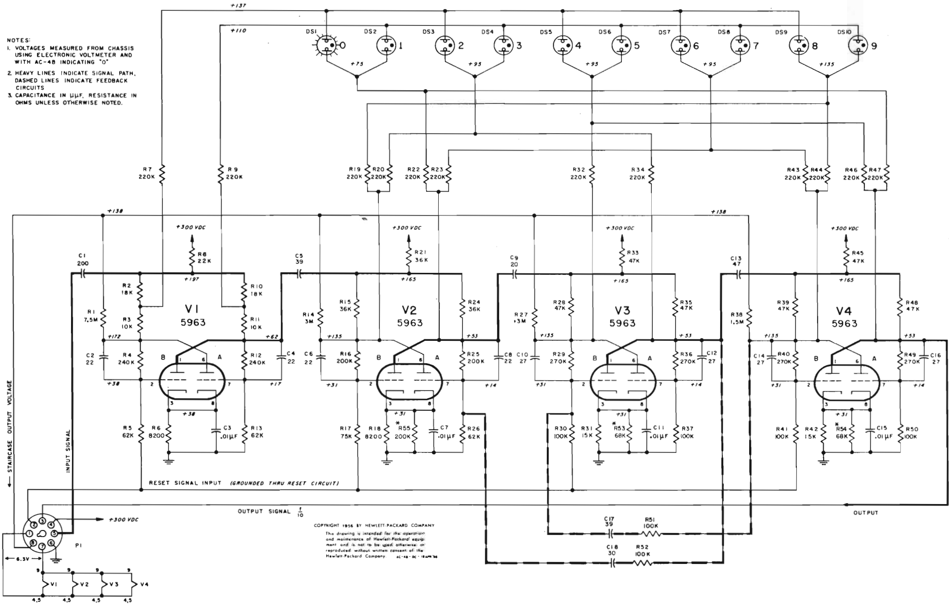
Figure 9. Model AC-4B Decade Counter
